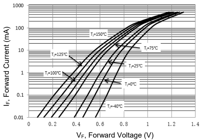
Fig 4. Forward Characteristics
