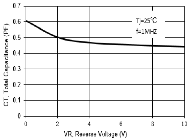
Fig 2. Capacitance Characteristics
