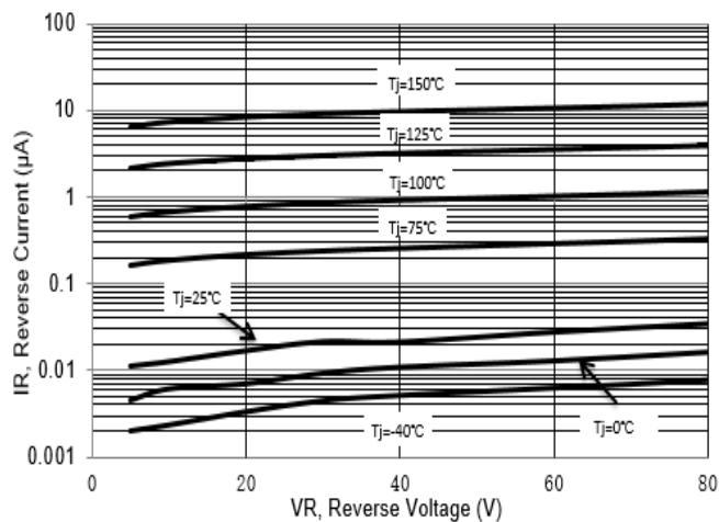
Fig 3. Reverse Characteristics
