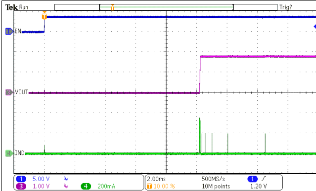
图 56. Start-up/Shutdown into No Load
