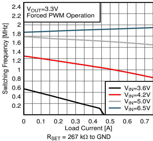
图 40. Switching Frequency versus Load Current V OUT = 3.3 V
