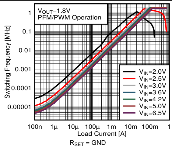
图 37. Switching Frequency versus Load Current V OUT = 1.8 V
