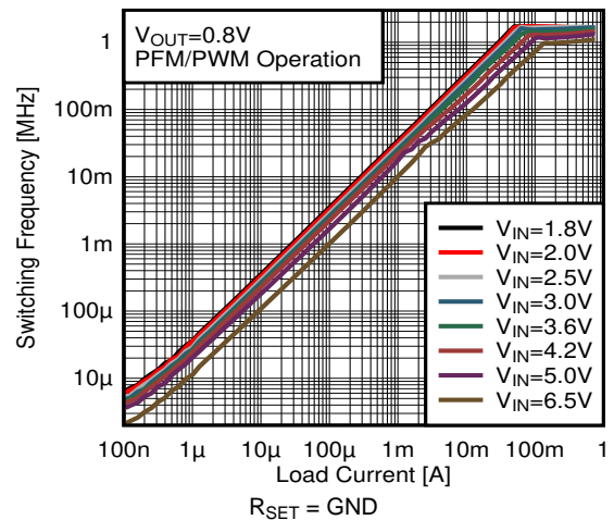
图 35. Switching Frequency versus Load Current V OUT = 0.8 V
