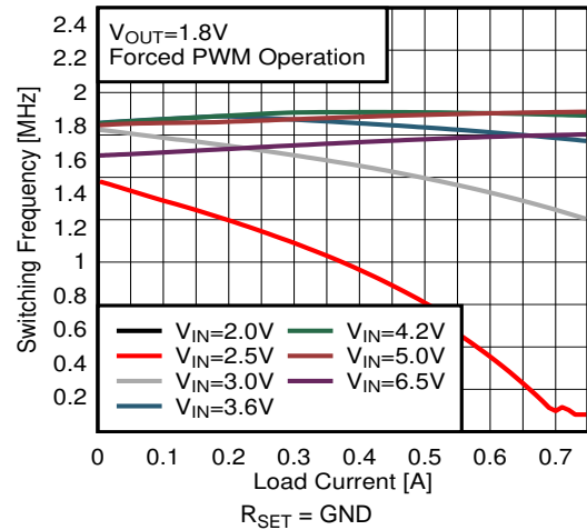
图 39. Switching Frequency versus Load Current V OUT = 1.8 V
