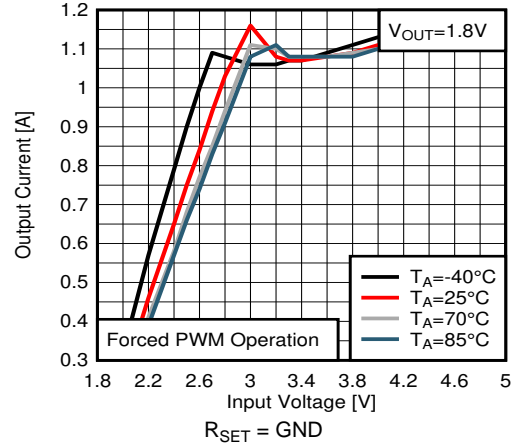
图 33. Maximum Output Current versus Input Voltage V OUT = 1.8 V
