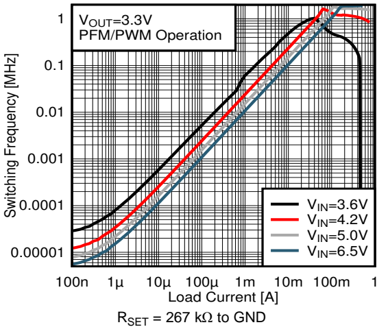
图 38. Switching Frequency versus Load Current V OUT = 3.3 V
