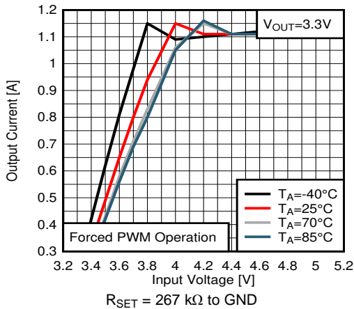
图 34. Maximum Output Current versus Input Voltage V OUT = 3.3 V
