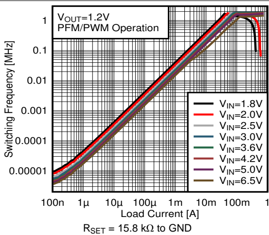
图 36. Switching Frequency versus Load Current V OUT = 1.2 V
