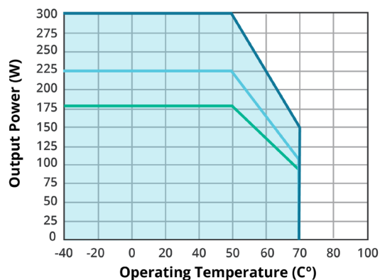
TEMPERATURE DERATING CURVE (12 Vdc output models)
