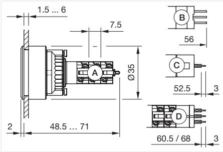
Dimensions [mm] A = Solder terminal B = Plug-in terminal 2.8 x 0.5 mm C = Universal terminal 2.0 mm x 0.5 mm Universal-Solder terminal
