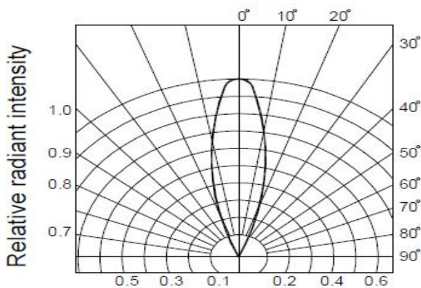
角度图/Directivity Diagram
