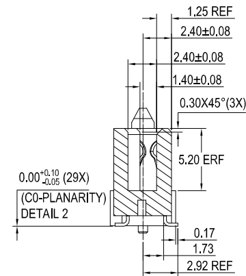
SECTION Y-Y
