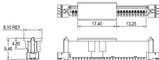
PART WITH PICK-UP CAP,SEE NOTE 4 SCALE 2:1
