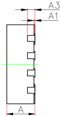
SIDE VIEW [侧视图]
