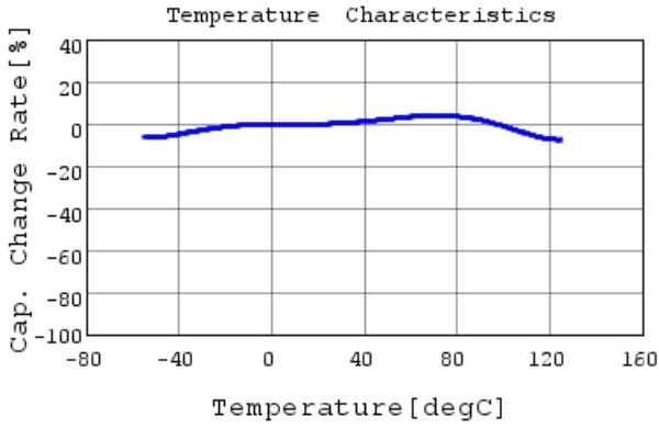
GRM188R71A225ME15 C-Temp. capchange, DC0.0V,
