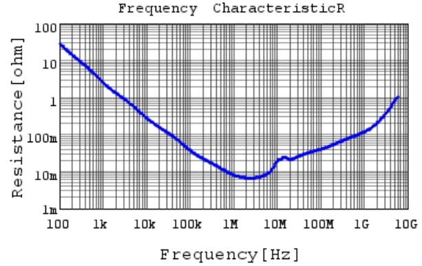
GRM188R71A225ME15 R DCOV, 25degC
