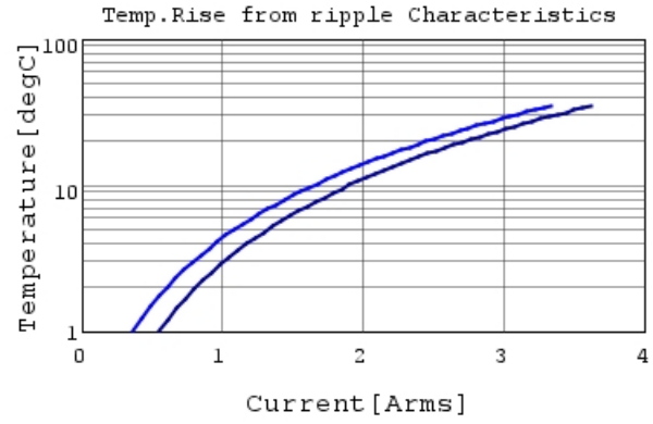
GRM188R71A225ME15 Temp.rise — 500kHz —
