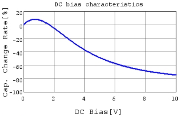
GRM188R71A225ME15 C-DC bias capchange, 25.0c
