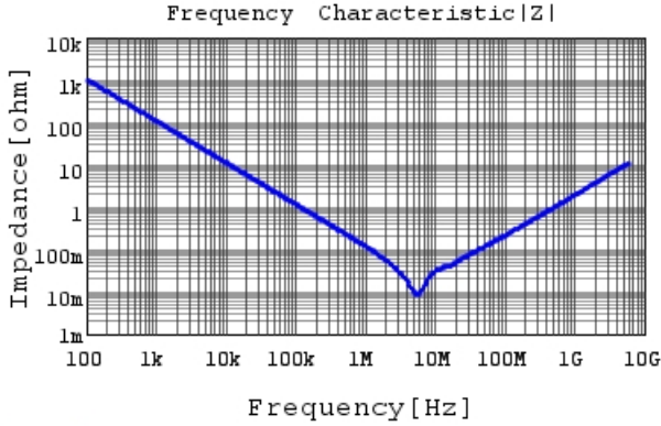
GRM188R71A225ME15 |Z| DCOV, 25degC
