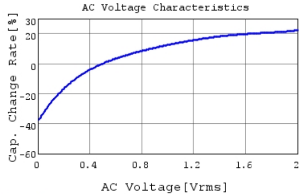
GRM188R71A225ME15 C-AC Voltage capchange, Dc
