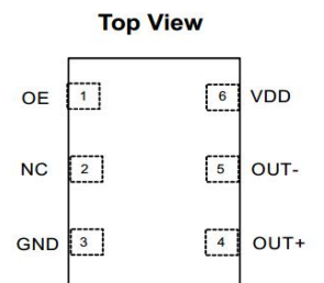
Figure 1. Pin Assignments
