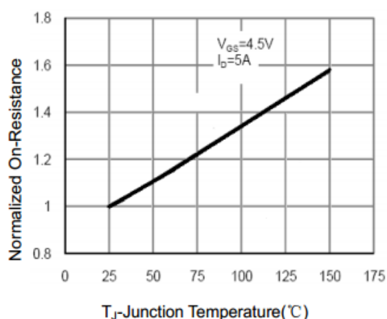
Figure 6 Drain-Source On-Resistance
