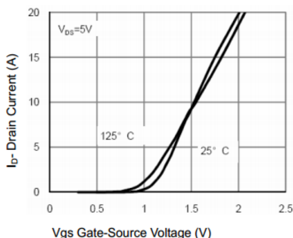
Figure 4 Transfer Characteristics
