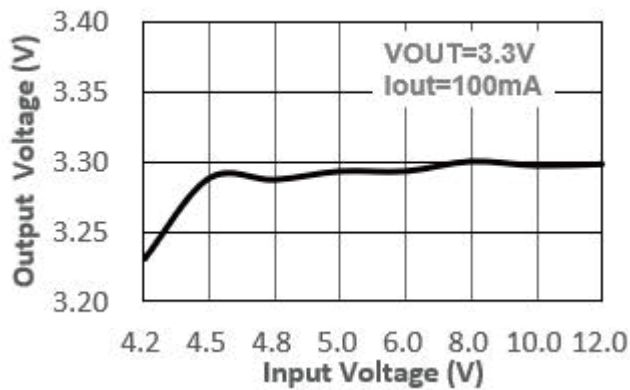
Output Voltage vs. Input Voltage (VOUT=3.3V)
