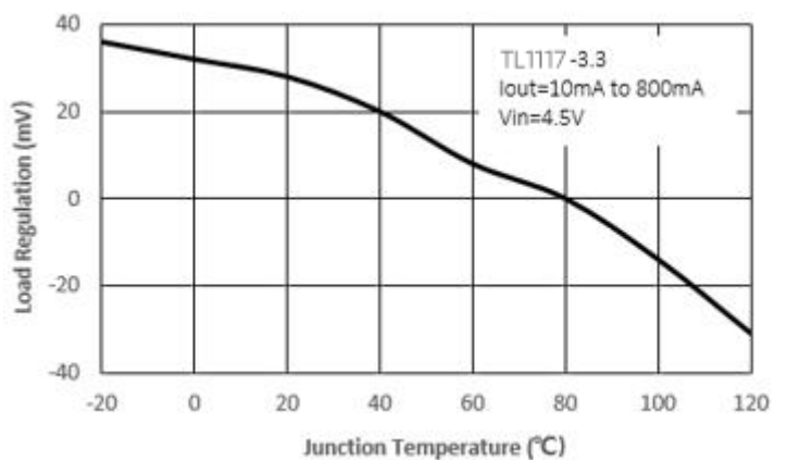
Load Regulation vs. Junction Temperature
