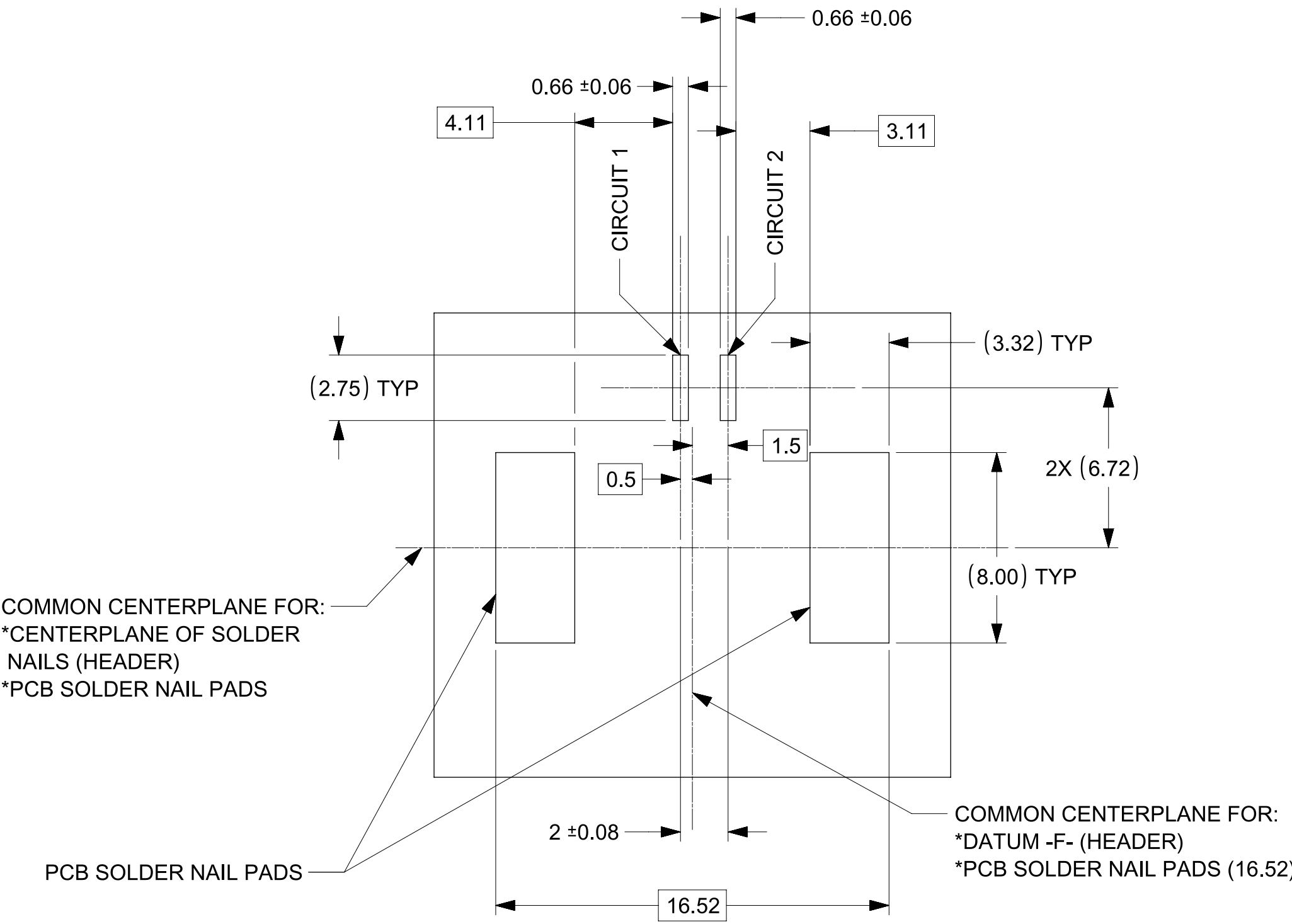
PCB LAYOUT
