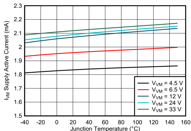
图 7-4. Active Current ( I_{VM} ) vs. Junction Temperature ( T_J )
