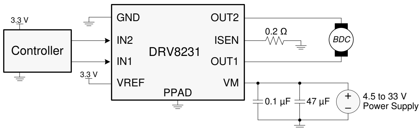
图 9-1. Typical Connections
