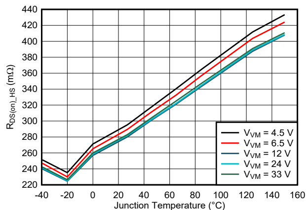
图 7-6. High-Side R_{DS(on)} vs. Junction Temperature ( T_J )
