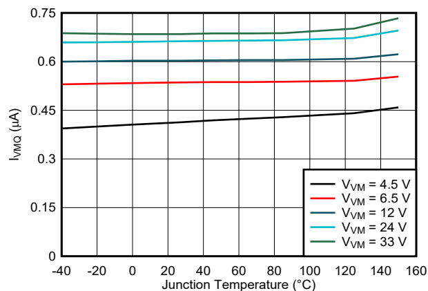
图 7-2. Sleep Current ( I_{VMQ} ) vs. Junction Temperature ( T_J )
