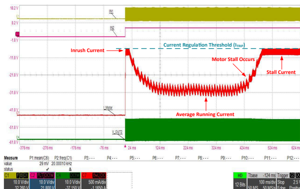
图 9-5. Motor startup at 50% duty cycle with current regulation
