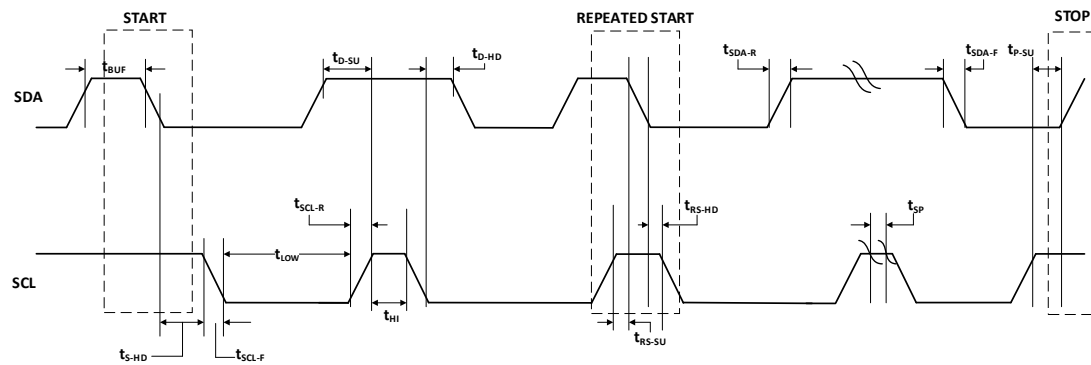
Figure 1 I²C Communication Port Timing Diagram
