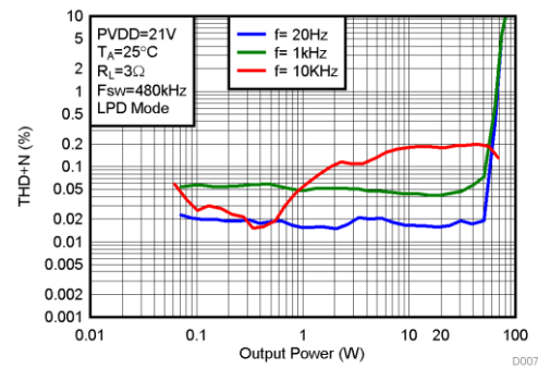
Figure 30 THD+N vs Output Power
