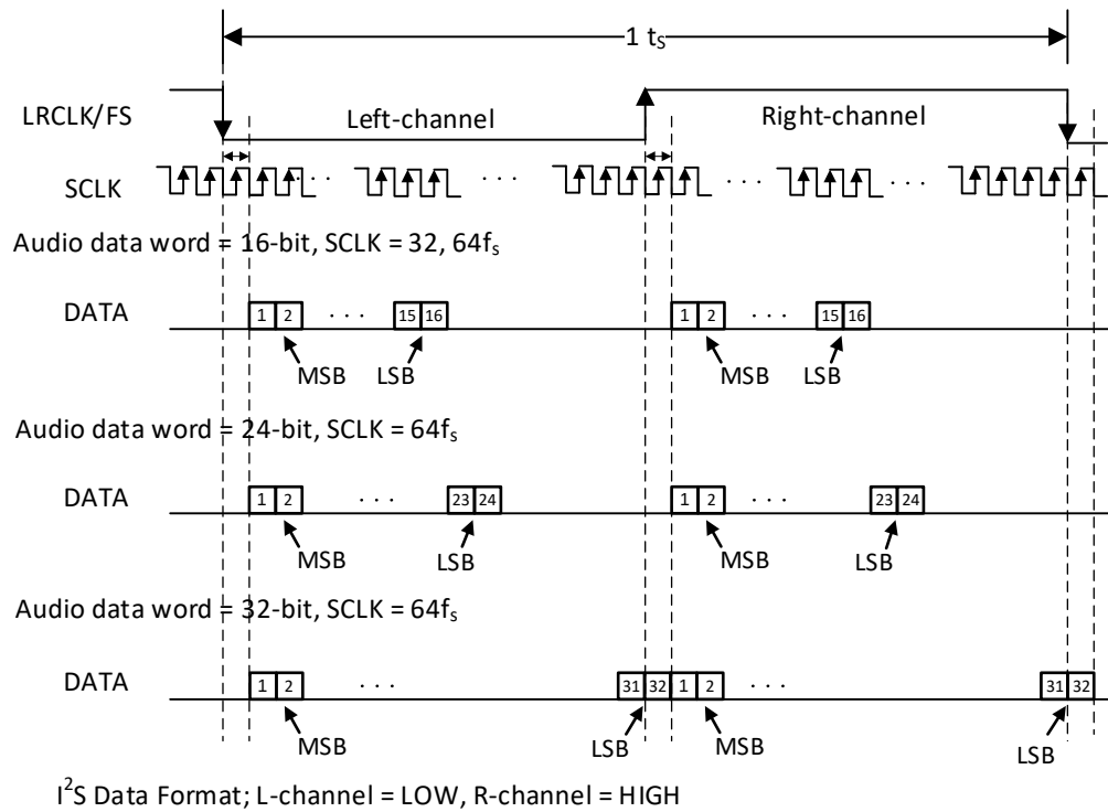
Figure 34 I²S Audio Data Format
