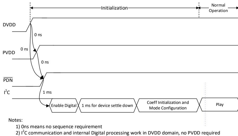
Figure 42 Start-up Sequence
