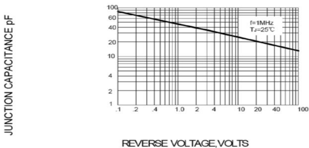
FIG.5-TYPICAL JUNCTION CAPACITANCE
