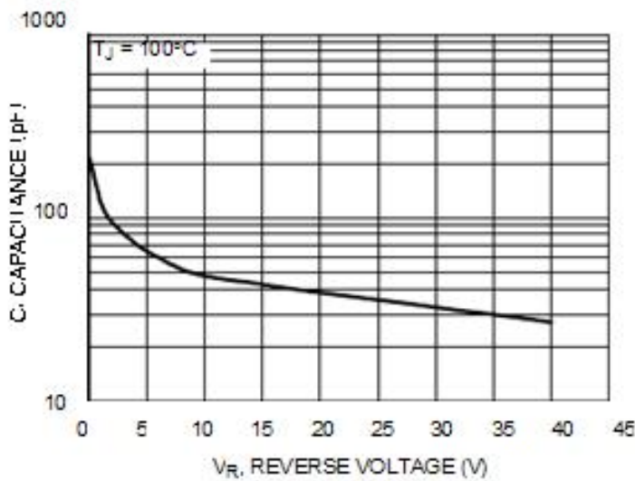
Figure 7. Capacitance
