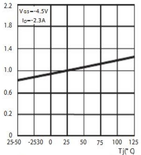
Figure 4. On-Resistance Variation with Temperature
