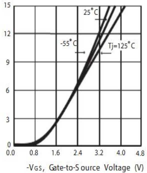
Figure 2. Transfer Characteristics
