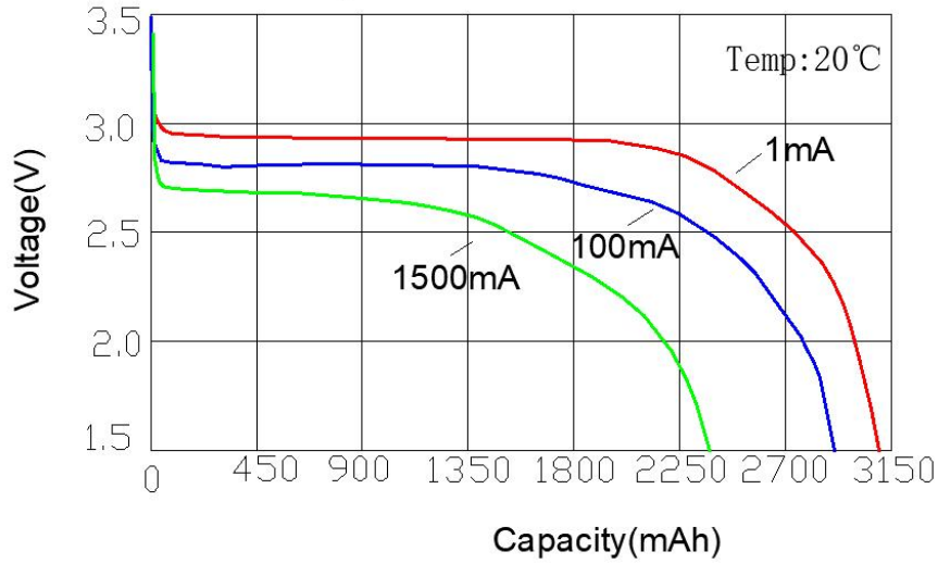
Discharge characteristics on current
