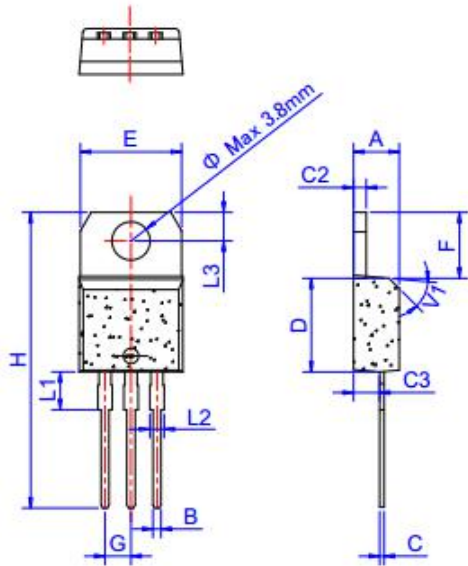
TO-220B
