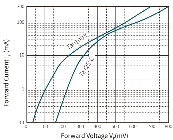
Fig.1 Forward Characteristics
