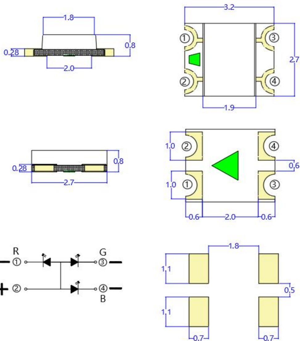
建议焊盘尺寸 Recommended Soldering Pattern
