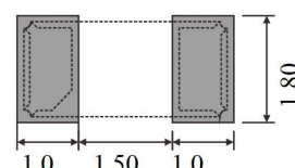
Recommended soldering Pattern
